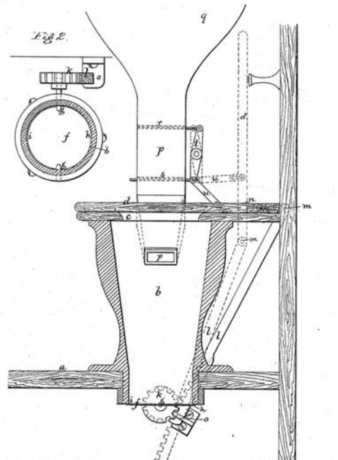
Water-Closets for Railroad-Cars. No. 147,363. Fig. 1. Patented Feb. 10, 1874.
